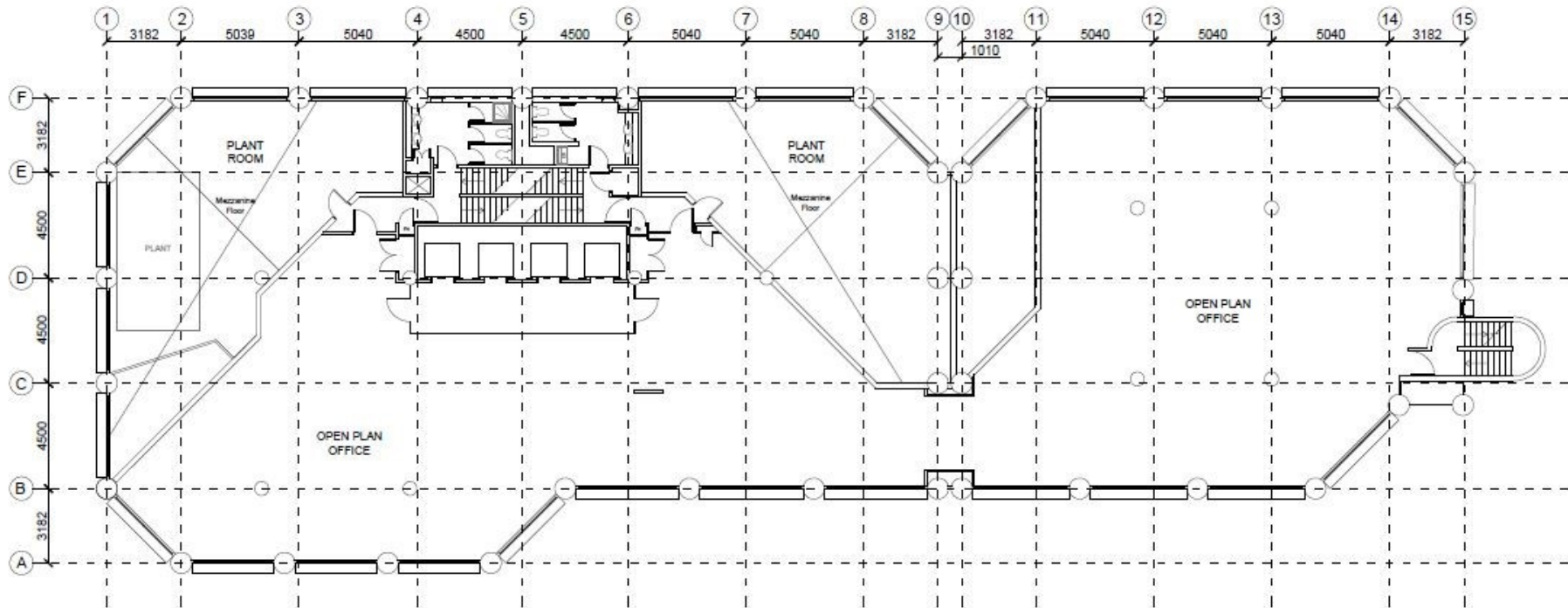
4 LEVEL 3 PLAN SCALE 1:100 @ A1 FLOOR AREA = 661.42m 2
